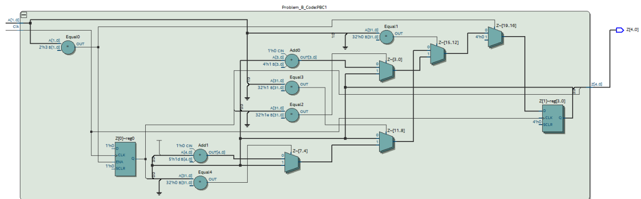
COUNTER EXPANDED RTL VIEW
