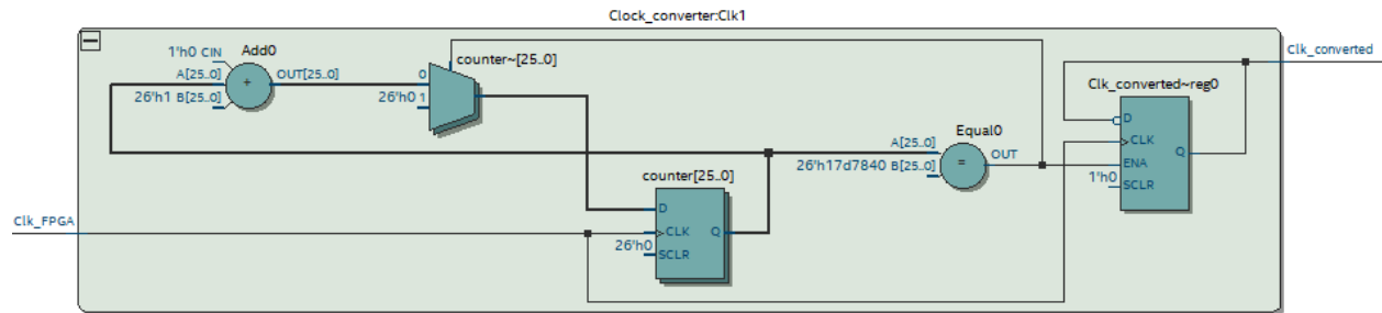
CLOCK_CONVERTER EXPANDED RTL VIEW
